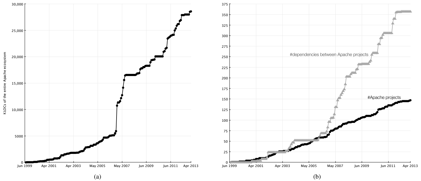
Fig. 2. Evolution of projects and dependencies (a) and size (b) in the Apache ecosystem.
