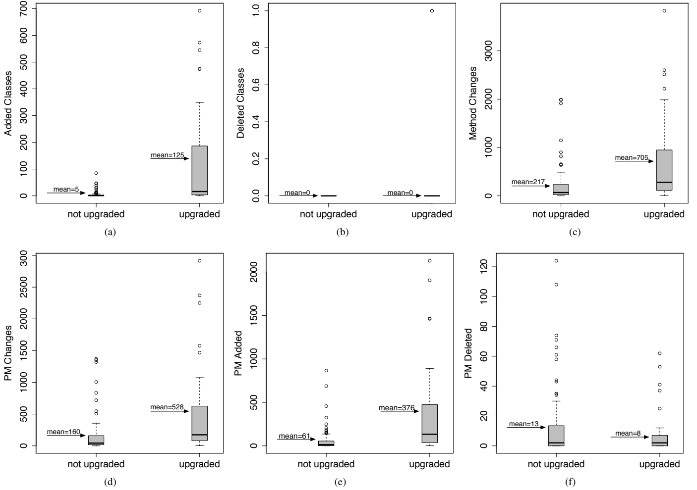
Fig. 4. Changes in upgraded and not upgraded releases.
